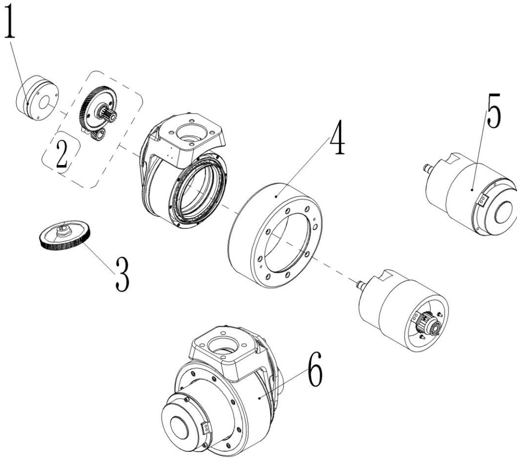
Fig. 5 Driving Wheel Components
